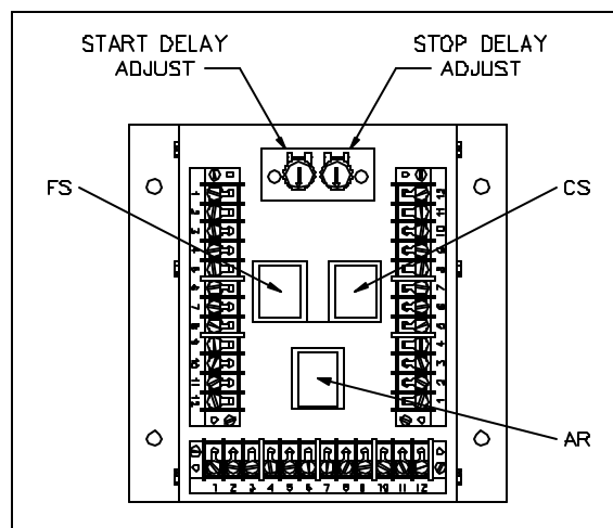
Figure 1 C122D/C242D Genset Control Module
